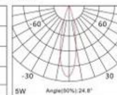
5W Angle(50%): 24.8°
