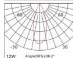
12W Angle(50%): 36.2°
