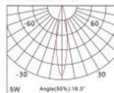
5W Angle(50%): 18.3°
